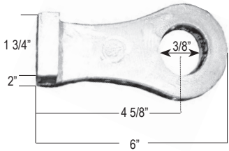
Adjustable Mount Bracket Detail
