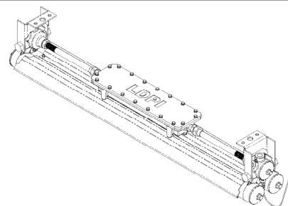
Drop mount kit 2 or 3 lamp P/N 4405 4 lamp P/N 4403
