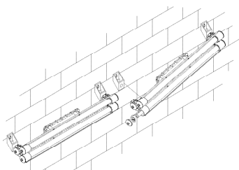
Wall/Ceiling mount kit For 2 or 3 lamp P/N 4401
